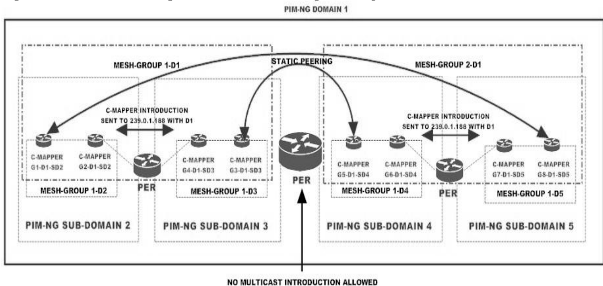
Figure 49 Mesh-Groups and C-MAPPER peering
