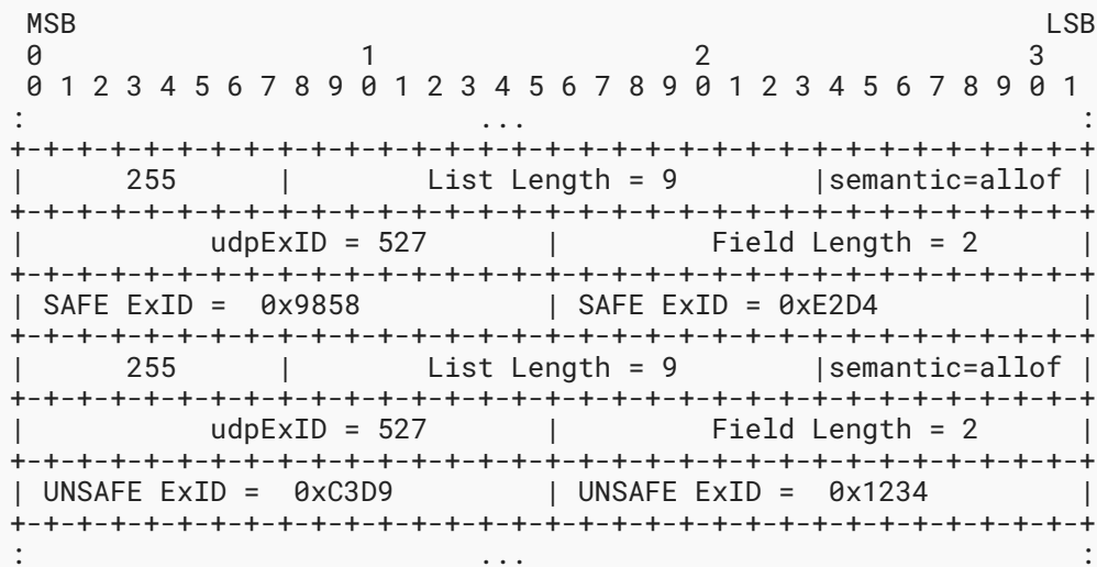
Figure 5: Example of UDP Experimental Option ExID IEs
