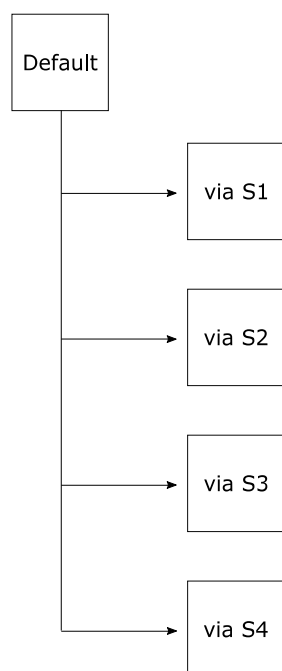
Figure 21: Abstract RIB
