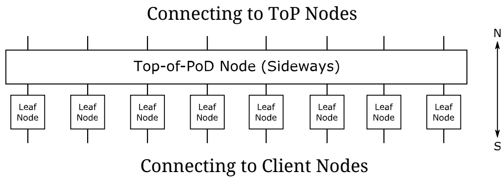
Figure 7: Side View of a PoD, K_{TOP}=8 , K_{LEAF}=6
