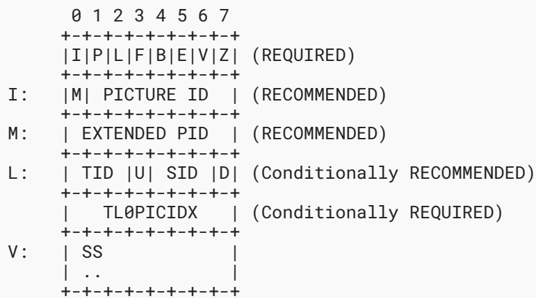
Figure 3: Non-Flexible Mode Format for VP9 Payload Descriptor
